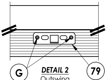
DETAIL 2 Outswing Multipoint Lock Strike Plate @ Sill
